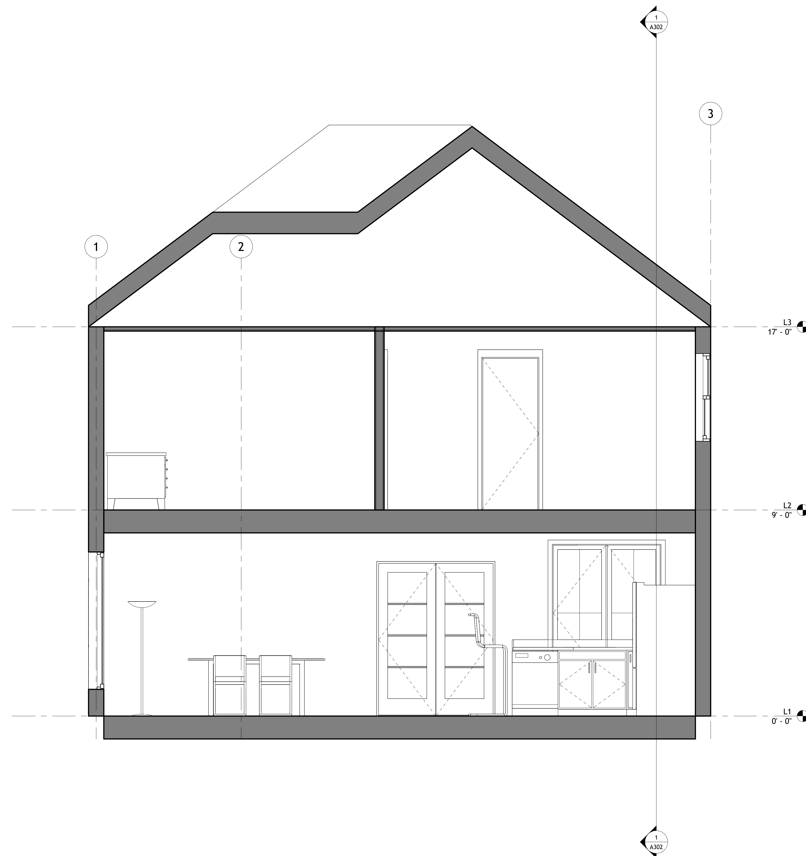
1 Section 2 1/2" = 1'-0"
